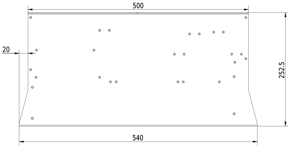
Dimensional drawing V800 - 45kW 4T0450
