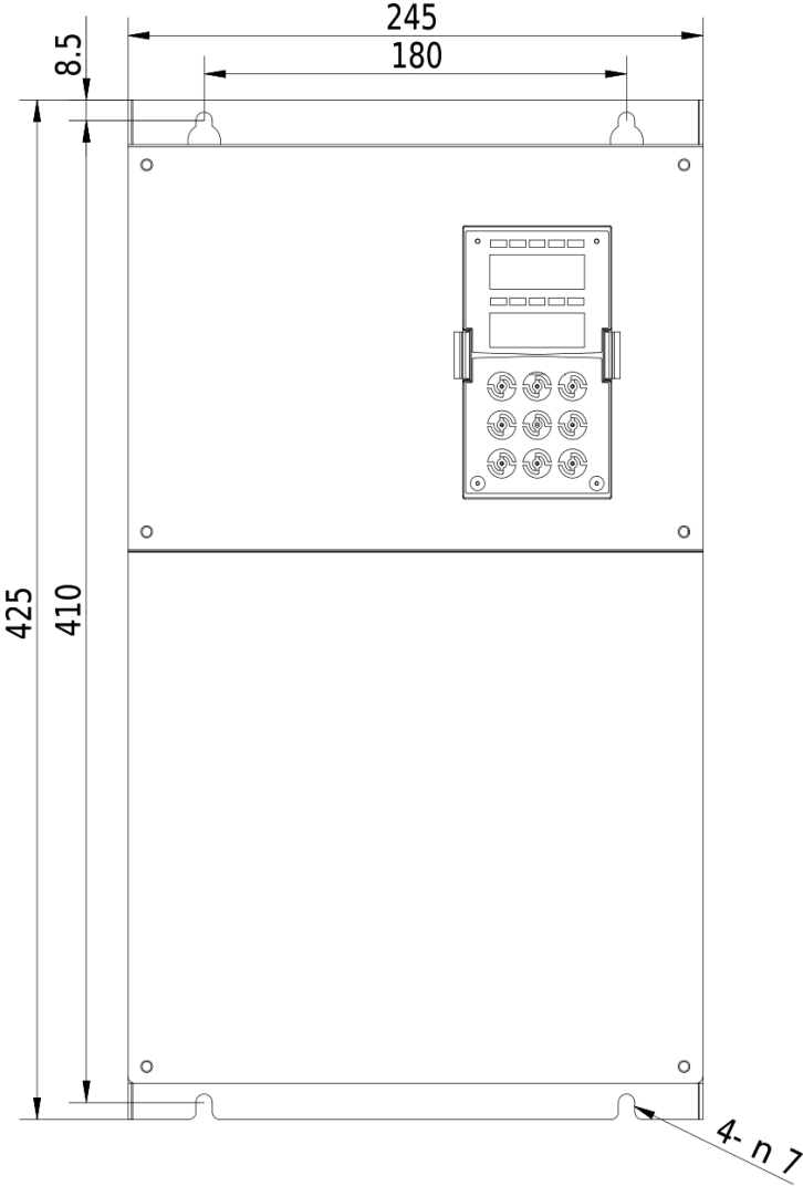
Dimensional drawing V800 - 37kW 4T0370
