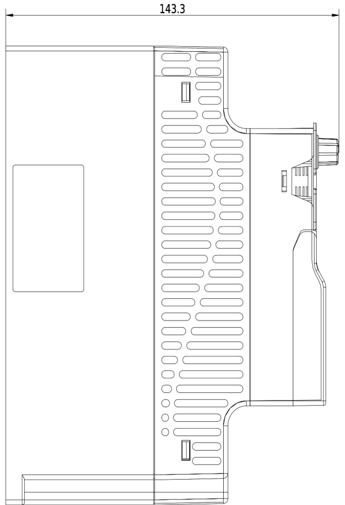
Dimensional drawing V800 - 3kW 2S0030
