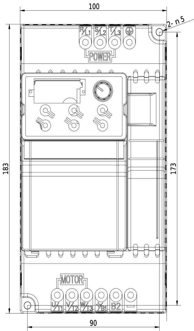
Dimensional drawing V800 - 3kW 2S0030
