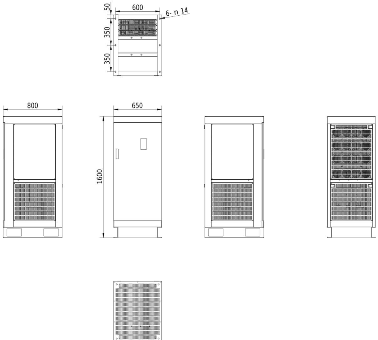
Dimensional drawing V810 - 710kW 4T7100
