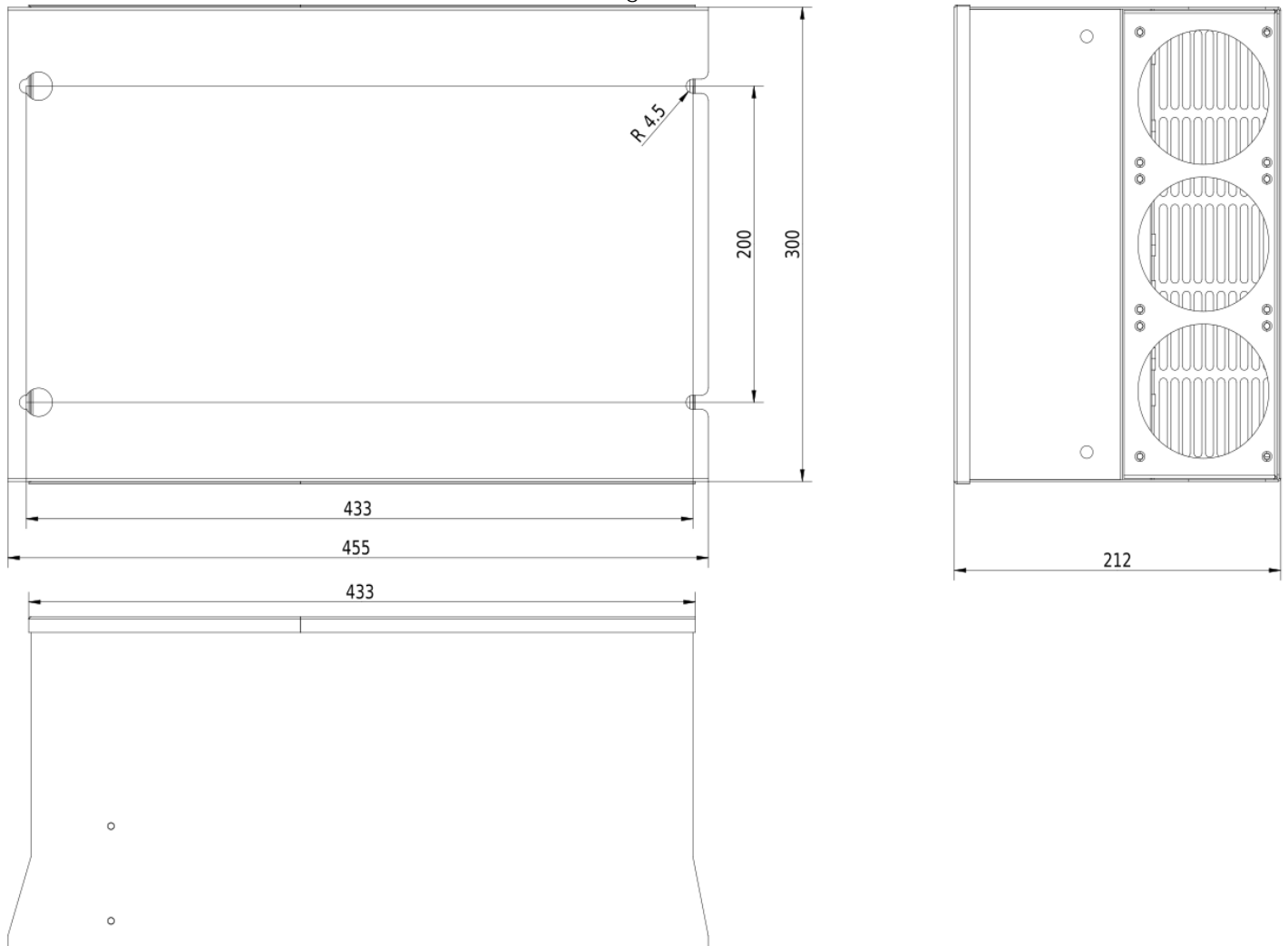
Dimensional drawing V810 - 45kW 4T0450
